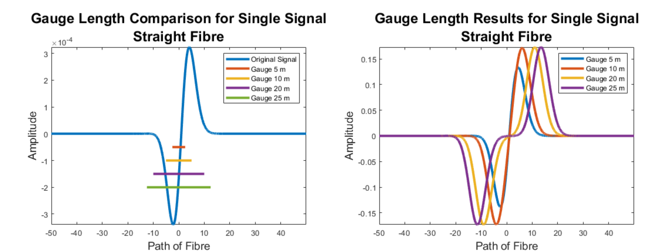
Figure 3: (Left) Comparison of the gauge lengths with respect to the full-waveform signal at t_1 of the straight fibre: (Blue) Original signal at t_1 (Red) Gauge length 5m, (Yellow) Gauge length 10m, (Purple) Gauge length 20m, and (Green) Gauge length 25m. (Right) Comparison of the gauge lengths applied to the full-waveform signal at t_1 of the straight fibre: (Blue) Gauge length 5m, (Red) Gauge length 10m, (Yellow) Gauge length 20m, and (Purple) Gauge length 25m.
