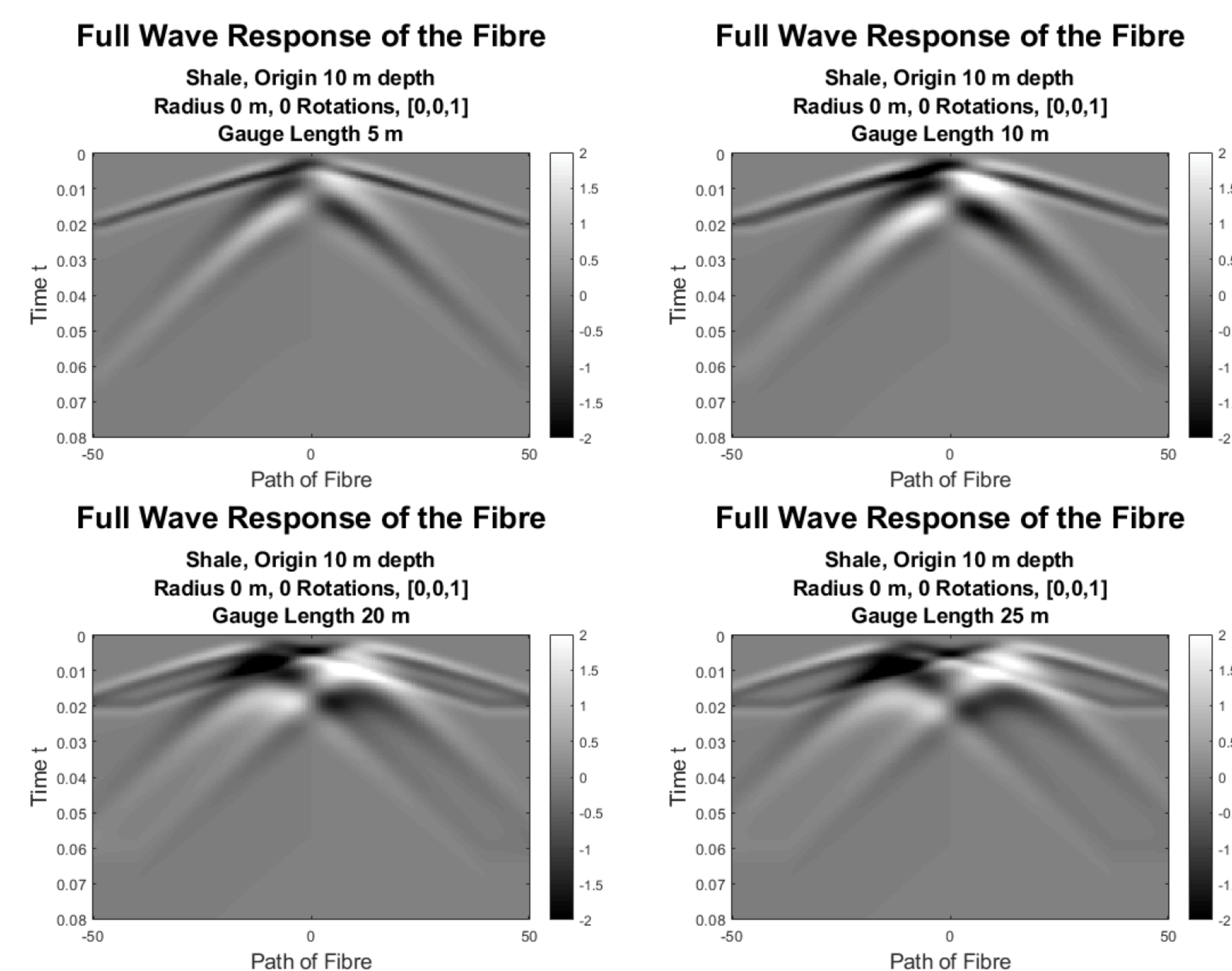
Figure 2: The full-wave response of the straight fibre in saturated shale when A = [0, 0, 1] for (top left) Gauge length 5 m, (top right) Gauge length 10 m, (bottom left) Gauge length 20 m, and (bottom right) Gauge length 25 m.
