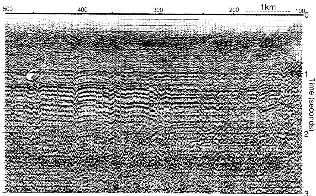
FIG. 4b. Radial (P-SV) component common-receiver stacked section without any statics applied.
