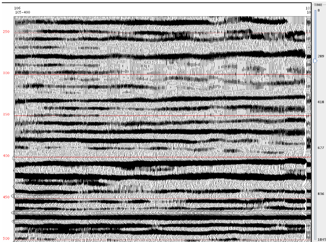
Figure 5: The noise attenuated CDP gather from Figure 4.
