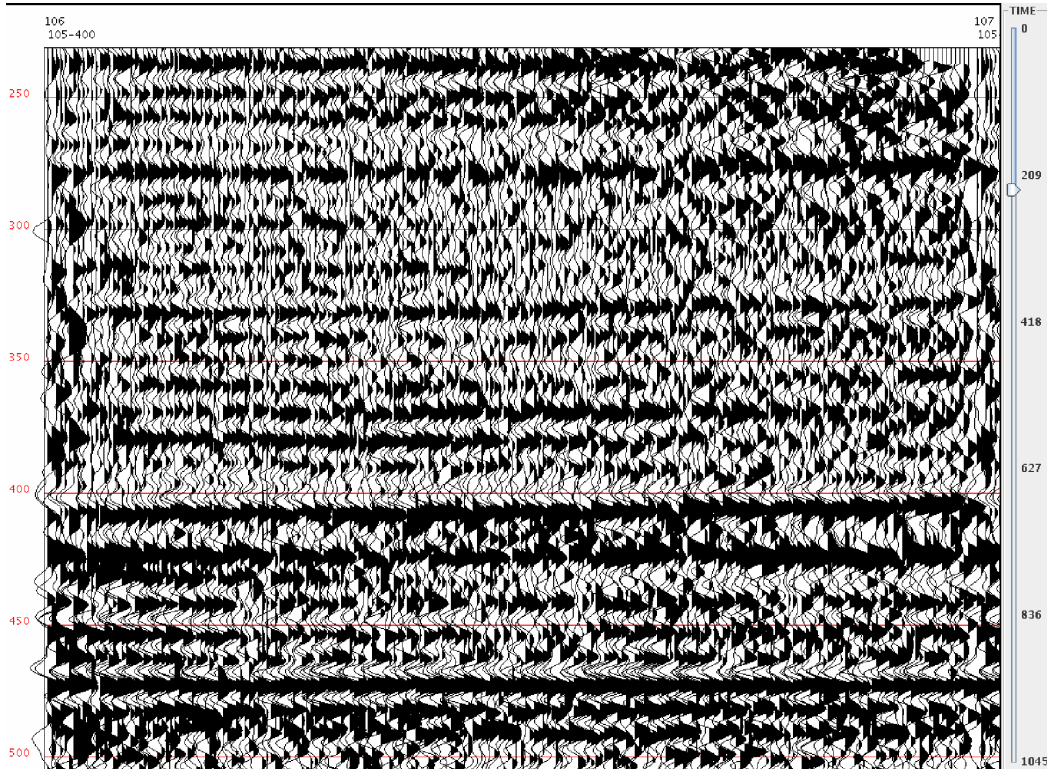
Figure 4: CDP NMO-corrected gather from Alberta oil sands.
